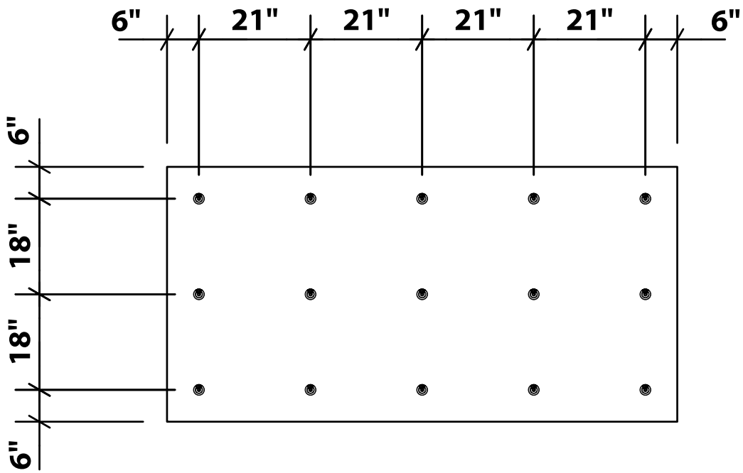
4' x 8'-(15) FASTENERS/BD. FM 1-105 PATTERN
