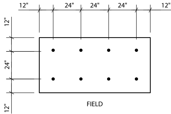
4' x 8'-(8) FASTENERS/BD.
